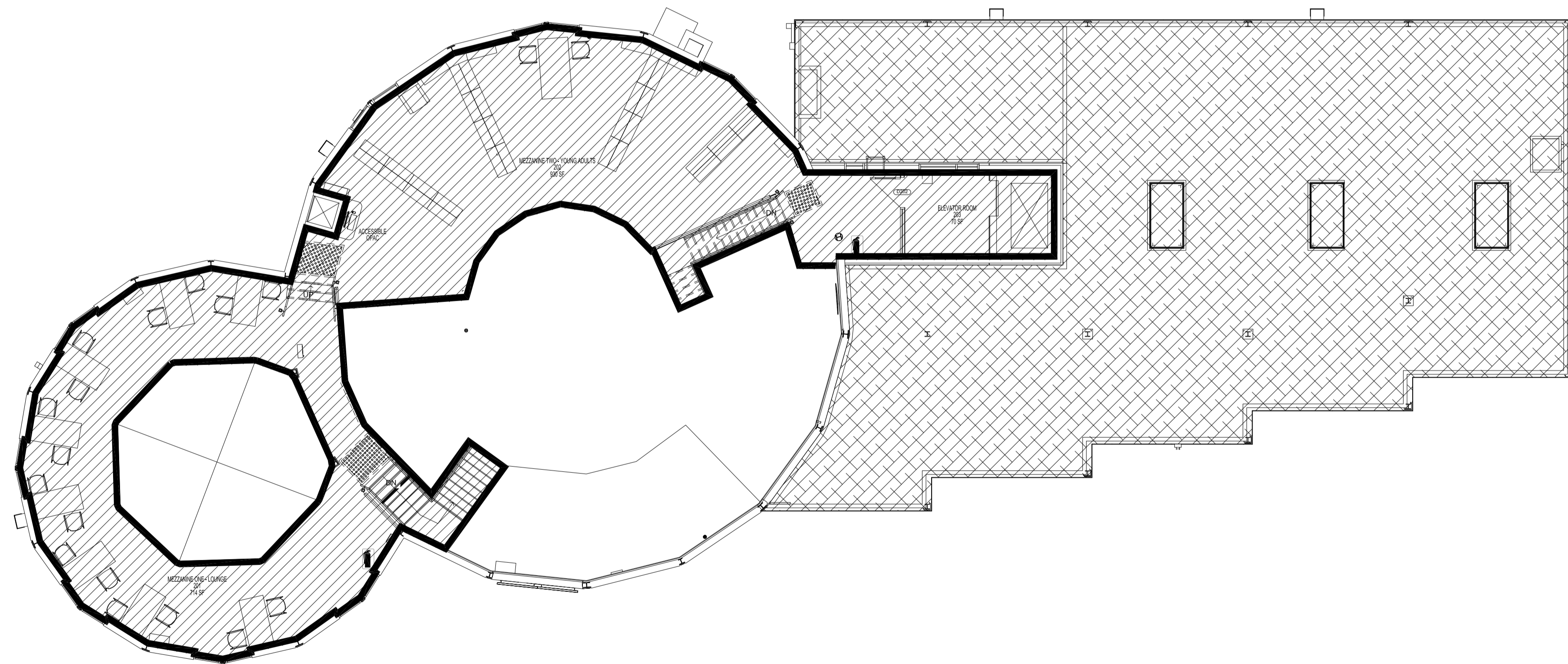
MEZZANINE FLOOR PLAN SCALE 1:100
